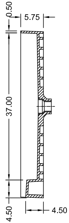
SECTION B-B
